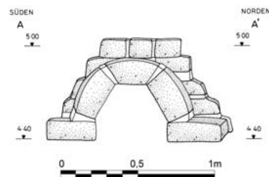
Abb. 130 F/I-j/21-Grav 14, Schnitt A–A'
